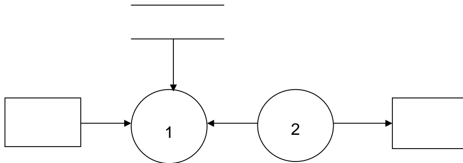
Gambar 1. Contoh proses
